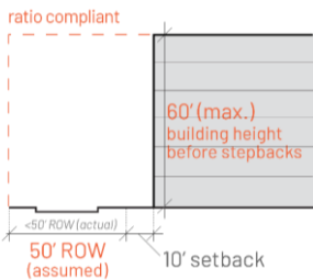
Figure 608-C. Narrow Right-of-Way Adjustment
