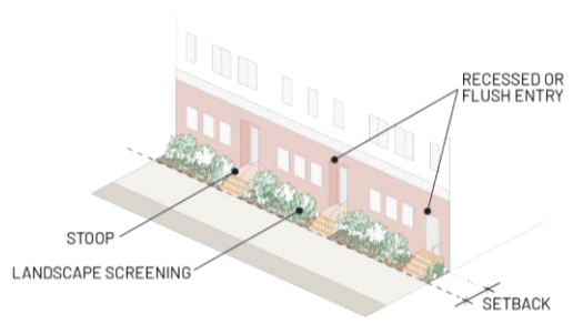
Figure 604-L. Stoop Frontage
