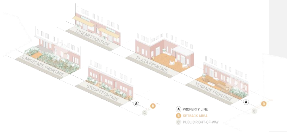
Figure 604-F. Frontage Types
