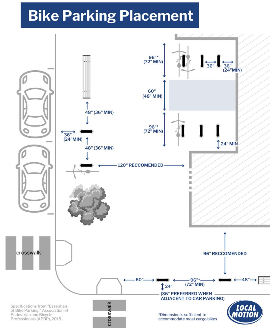
Figure 3: Bike Rack Placement (e) Bicycle parking serving buildings with multiple entrances shall be dispersed so that all principal entrances are served. (f) For office building use, up to 50% of short term bicycle parking requirements may be met by supplementing the (indoor) long term bicycle parking requirements with the required short term
