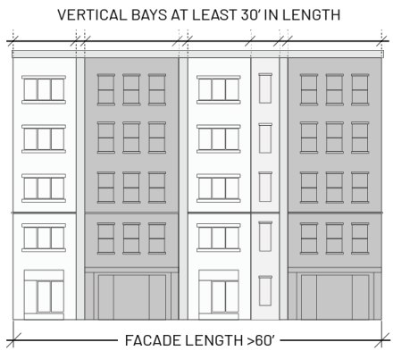
Figure 608-O. Vertical Articulation
